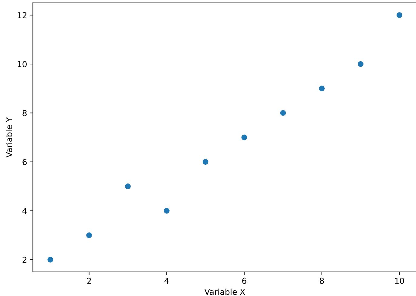
Scatter Plot
