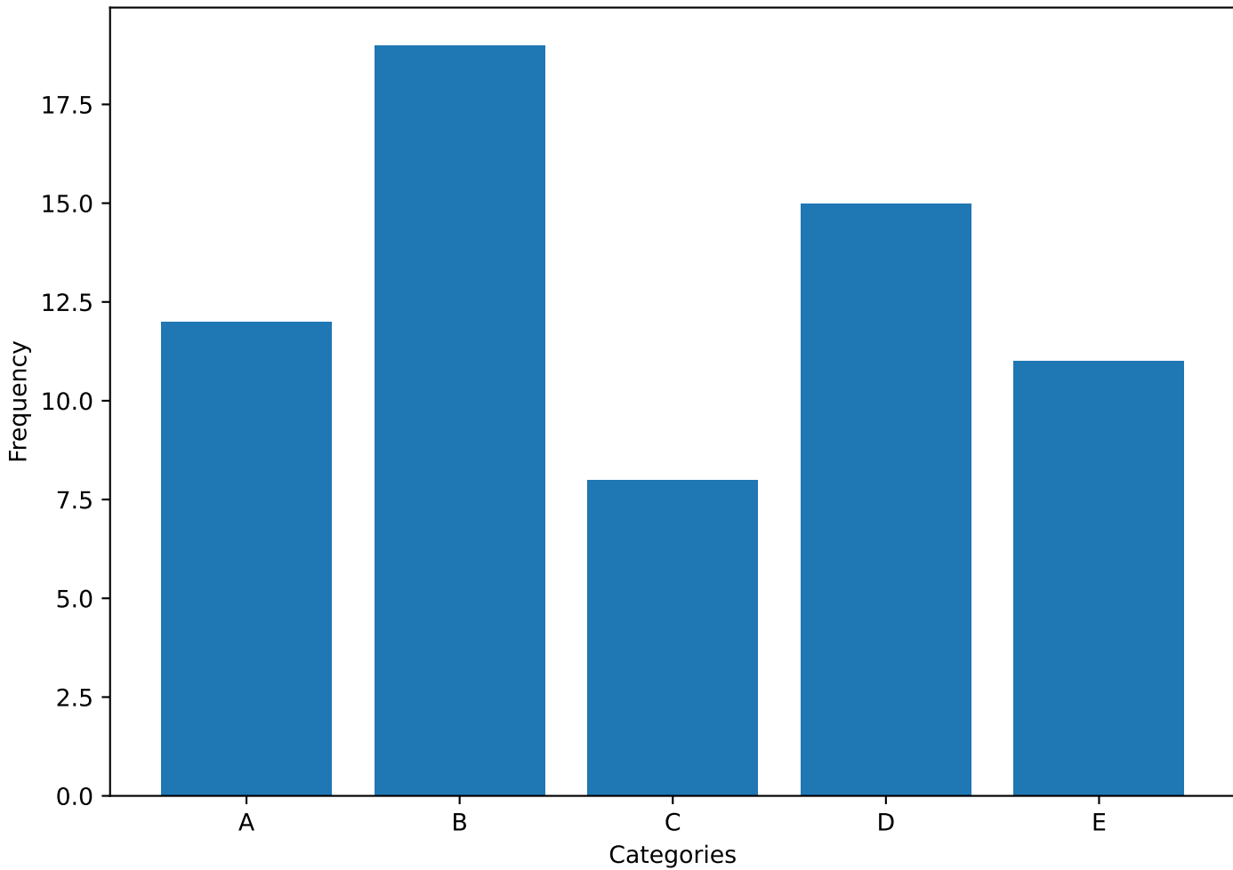
Bar Chart
