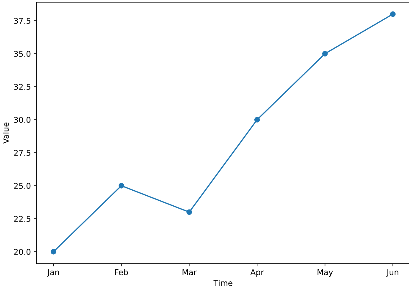
Line Graph
