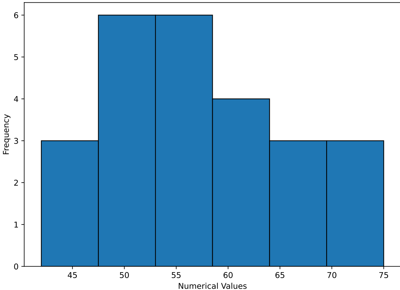
Histogram
