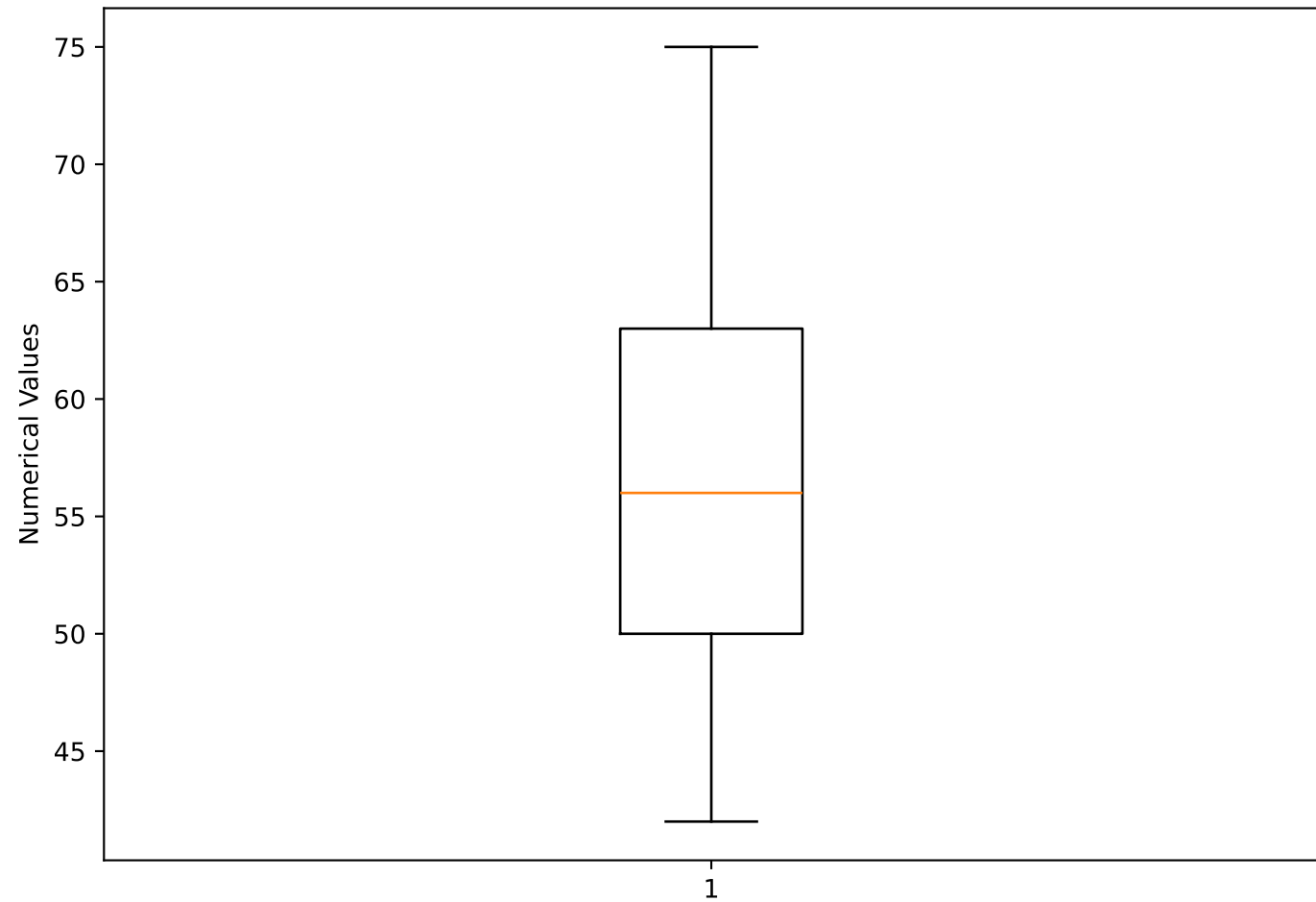
Box Plot
